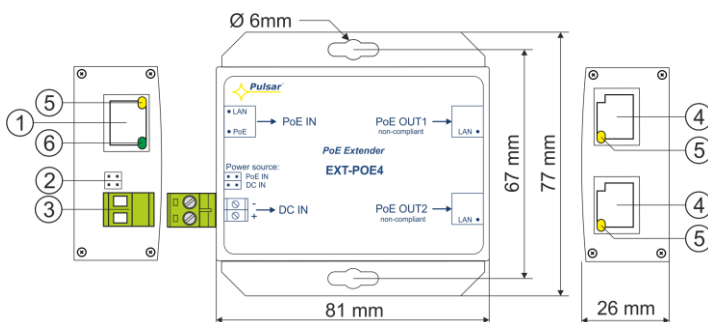
Fig.1. A schematic drawing of the device.
